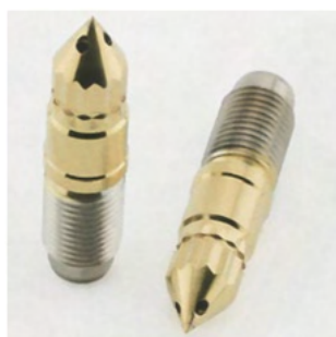
3551789: 6-hole; 5mm 3551791: 6-hole; 8mm
